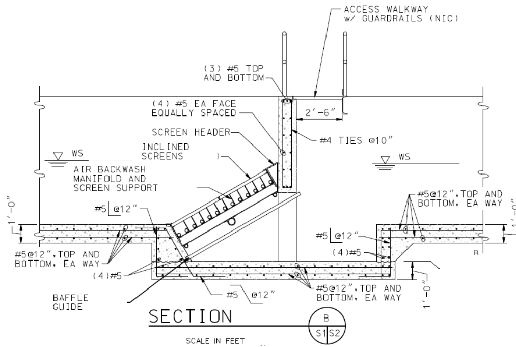
Figure 4-10 Typical Inclined Flat-Plate Screen
