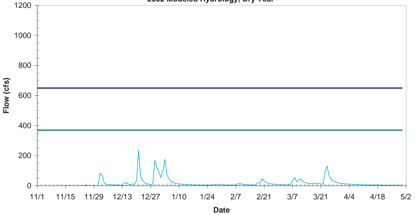
2002 Modeled Hydrology, Dry Year
